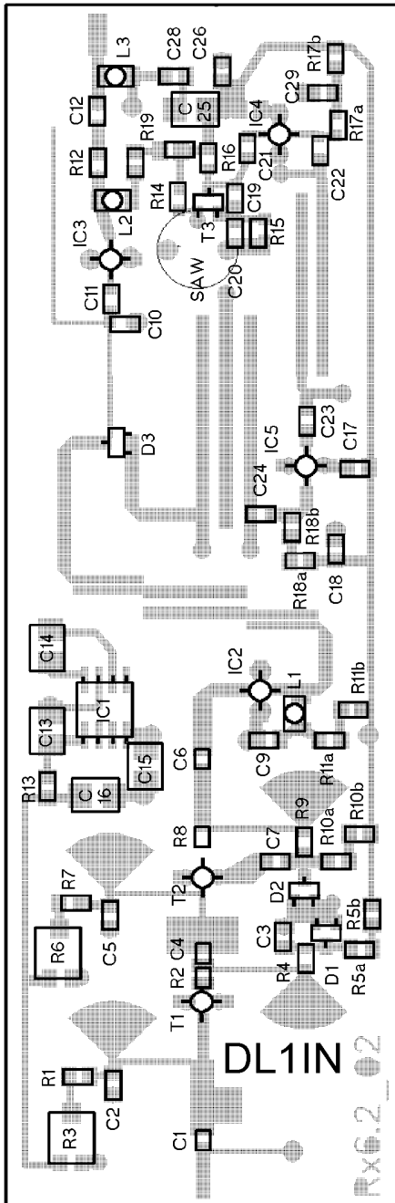
Fig. 4: Components Plan with SMD Components on Foil Side
