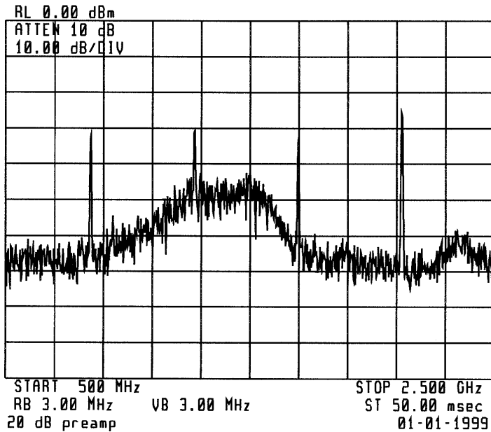
Fig. 2: Intermediate Frequency Spectrum of 5.7 GHz Converter without Input Signal
